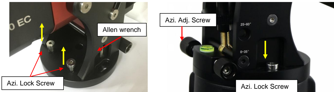
Figure 13. Attach the mount
