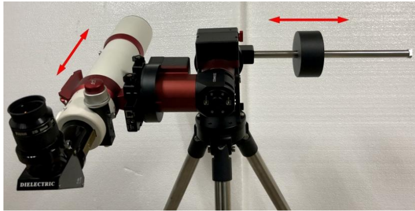
Figure 19. Balance a mount
